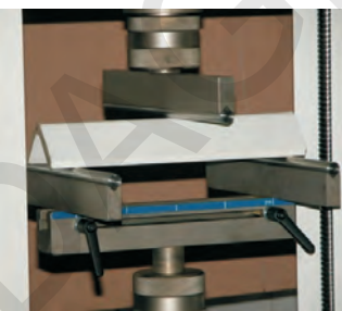
Deflection of paperboard angle plate
