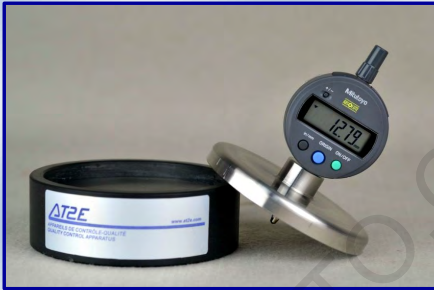
Supply with Zero-setting base
