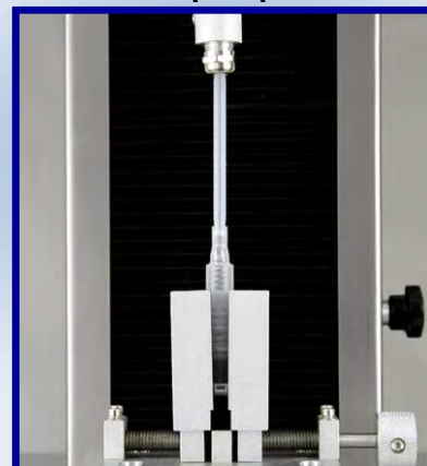
Push test of pump force
